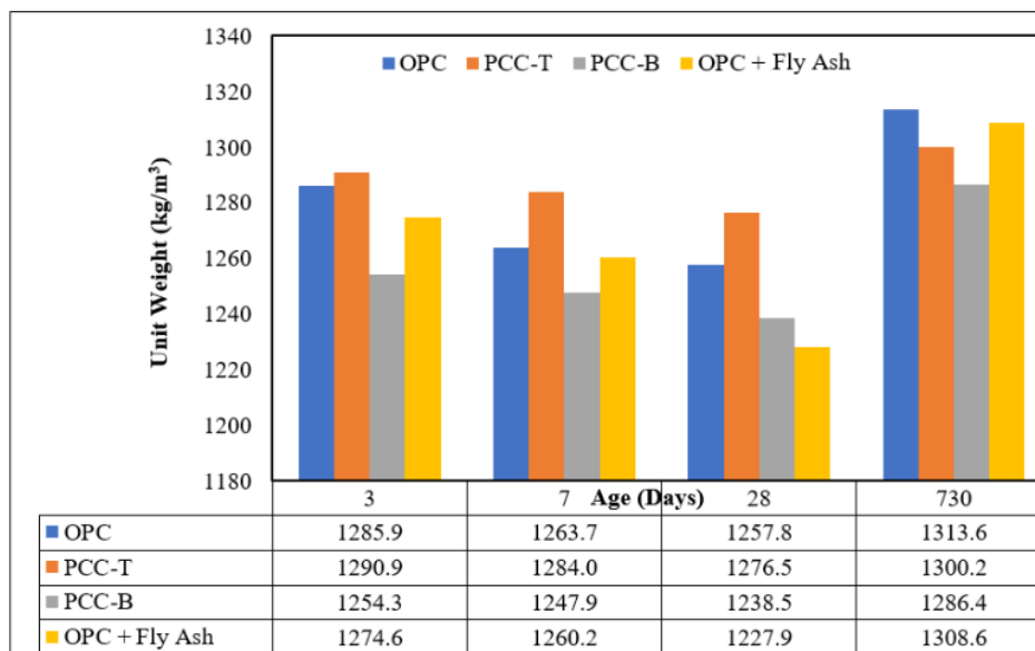
FIGURE 2. Unit weight test results
