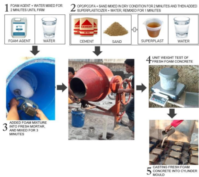
Figure 1. Foam Concrete mixture process
